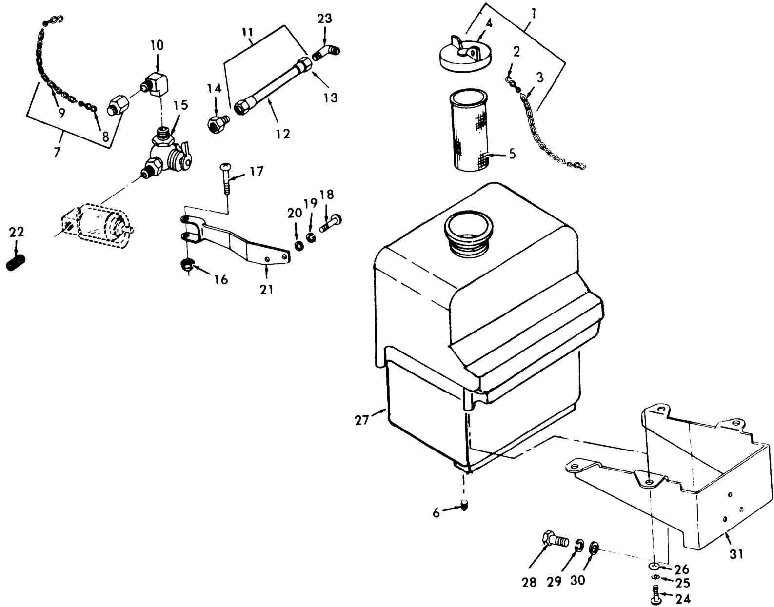
Figure 3. Fuel System
